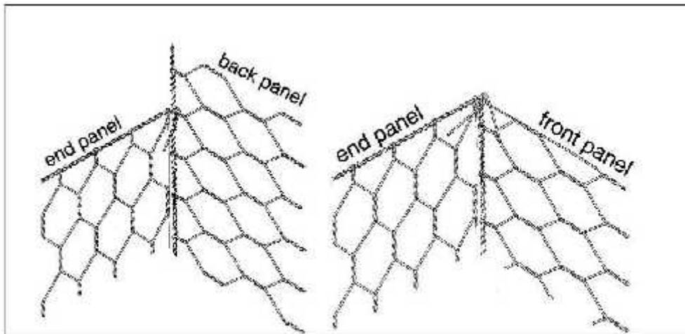
FIG. 3 Assembly—Gabions—Selvege Connection End and Front Panel to Back Panel
