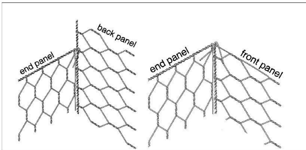
FIG. 3 Assembly—Gablons—Selvage Connection End and Front Panel to Back Panel
