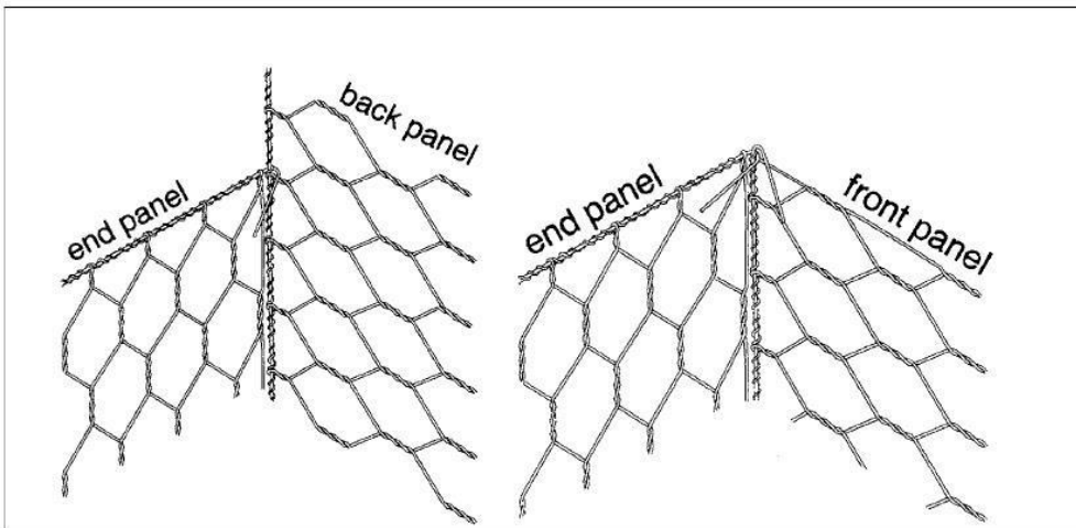
FIG. 3 Assembly—Gablons—Seldedge Connection End and Front Panel to Back Panel
