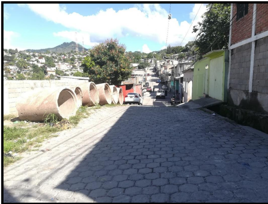
No.2 Vista general calle 1, se observan adoquines a remover.
