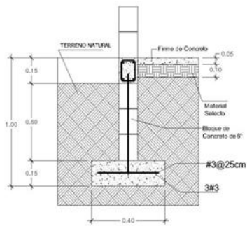
ZAPATA CORRIDA 0.40X0.15m
