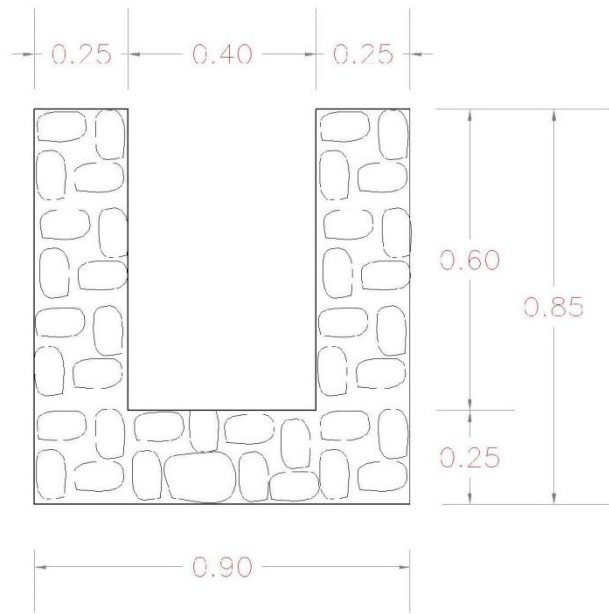
DETALLE CUNE A MAMPOSTERIA
