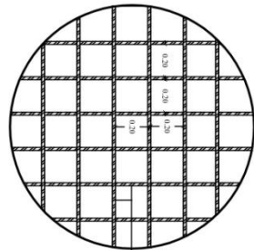
Armado Inferior Long. # 5 @ 20 cm Trans. # 5 @ 20 cm
